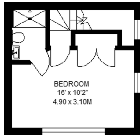
Upper Floor
